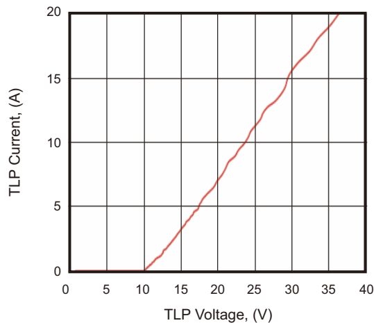
Fig.7 - Negative TLP IV Curve
